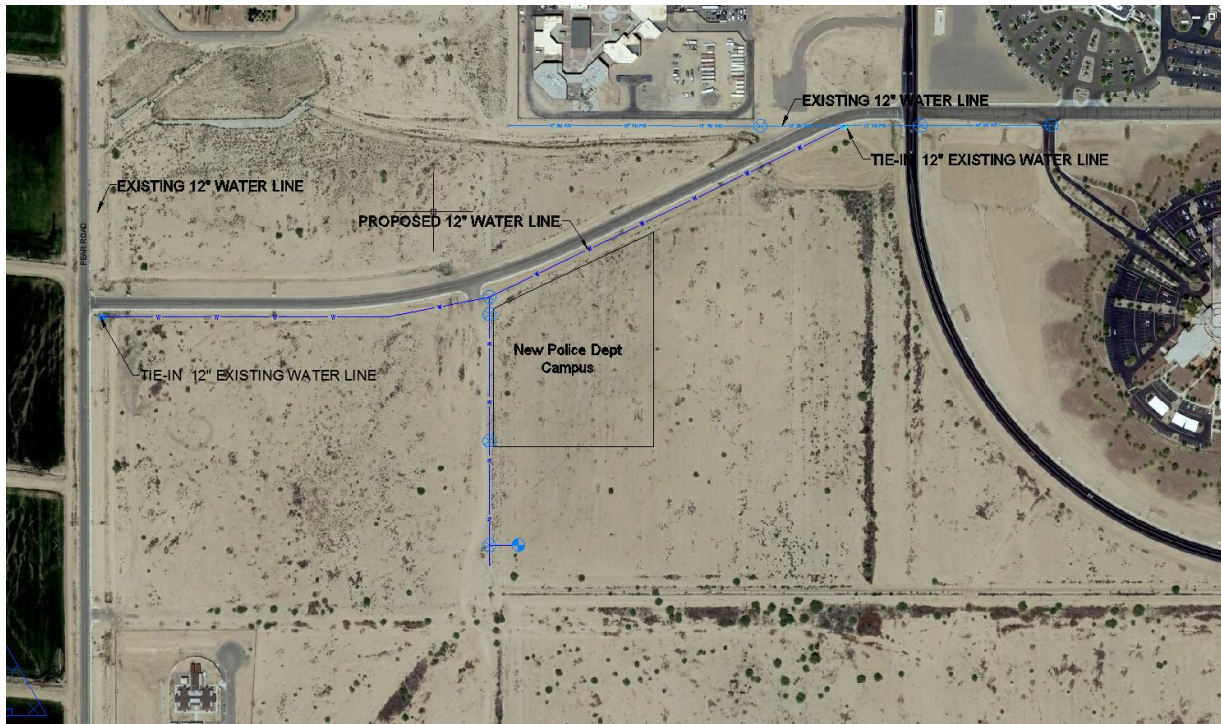
Figure 1: New 12" and 8" Water line Connection between Pear and Bluebird Rd (To be Installed)
